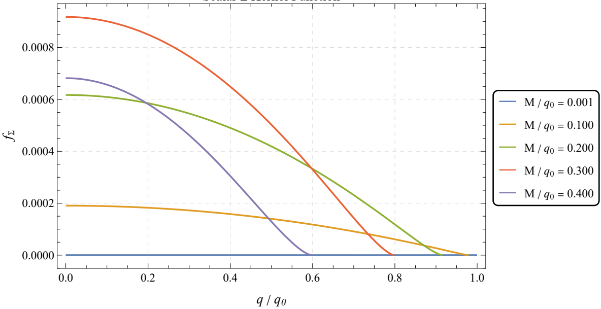
Scalar \Sigma Kernel Function
